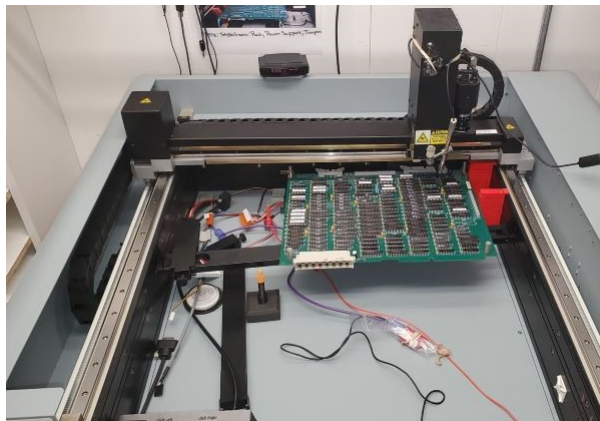
Huntron Flying Probe Test Bed
